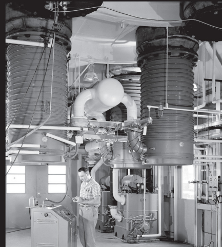
Interior of the Vacuum Pump House located directly below the Space Power Chambers' vacuum tank. The pump house had 10 oil diffusion pumps that could evacuate the chamber to pressure levels found in space at 100-mile altitude. The tunnel's existing exhausters removed most of the air in the chamber, then these diffusion pumps created the final vacuum levels. The vents, which can be seen in this photograph hanging from the ceiling, fed directly into the bottom of the chamber.
