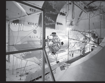
The first tests conducted in the new Space Power Chambers were a series of Atlas/Centaur retrorocket studies in September 1963. An Atlas/Centaur mass-model vehicle was placed horizontally on landing gear-type wheels in the larger test chamber with a net at the other end of the chamber to catch the Atlas mockup. After initial runs showed inconsistent behavior of the retrorockets, they were successfully redesigned by the manufacturer and qualified during another round of Space Power Chamber testing in 1964.
