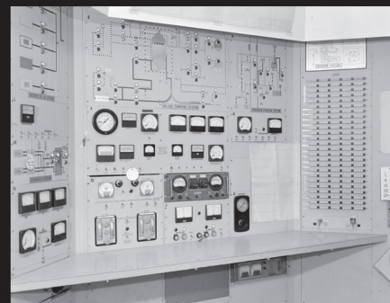
Centaur tanking controls in the Space Power Chambers' space tank control room, which was located underneath the former wind tunnel test section. This new control room was intended to replicate the Centaur controls in the launch room at Cape Canaveral. The former wind tunnel control room, located above on the mezzanine level, was used to control the tests conducted in the larger test chamber.
