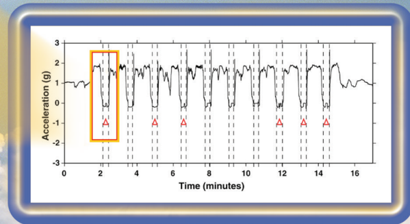
Acceleration levels experienced on a series of parabolic maneuvers.
