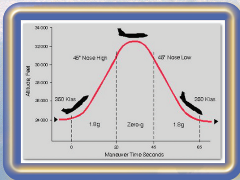
The KC-135 flies a series of parabolic maneuvers similar to a series of roller coaster hills.
