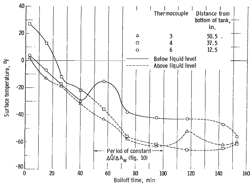
Figure 11. - Typical variations in surface temperatures during boiloff of liquid hydrogen from sealed-foam-insulated tank. (Thermocouple 5 was inoperative.)
