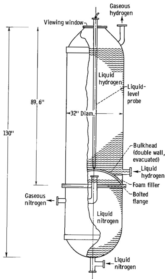
Figure 2. - Flight-weight propellant tank 2 used for insulation studies.
