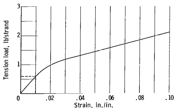
Figure 6. - Load-strain curve for single-strand nylon constrictive wrap.
