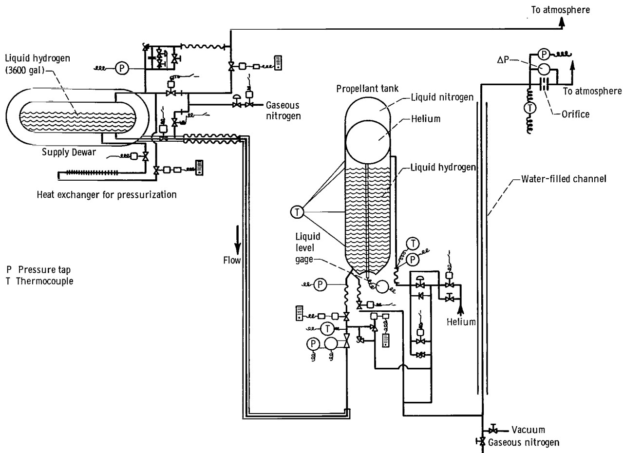
Figure 8. - Schematic of flow system instrumentation used for studies of insulation systems on liquid-hydrogen propellant tanks.
