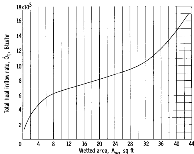
Figure 10. - Typical plot of total heat inflow rate against wetted area as determined from boiloff curve of figure 9.
