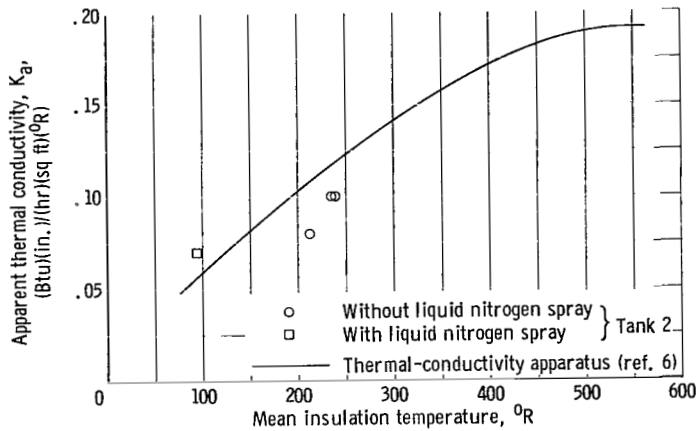
Figure 16. - Comparison of previous thermal-conductivity data and results for propellant tank 2 on sealed and constrictive-wrap Freon-blown polyurethane foam insulation with density of 2.5 pounds per cubic foot.
