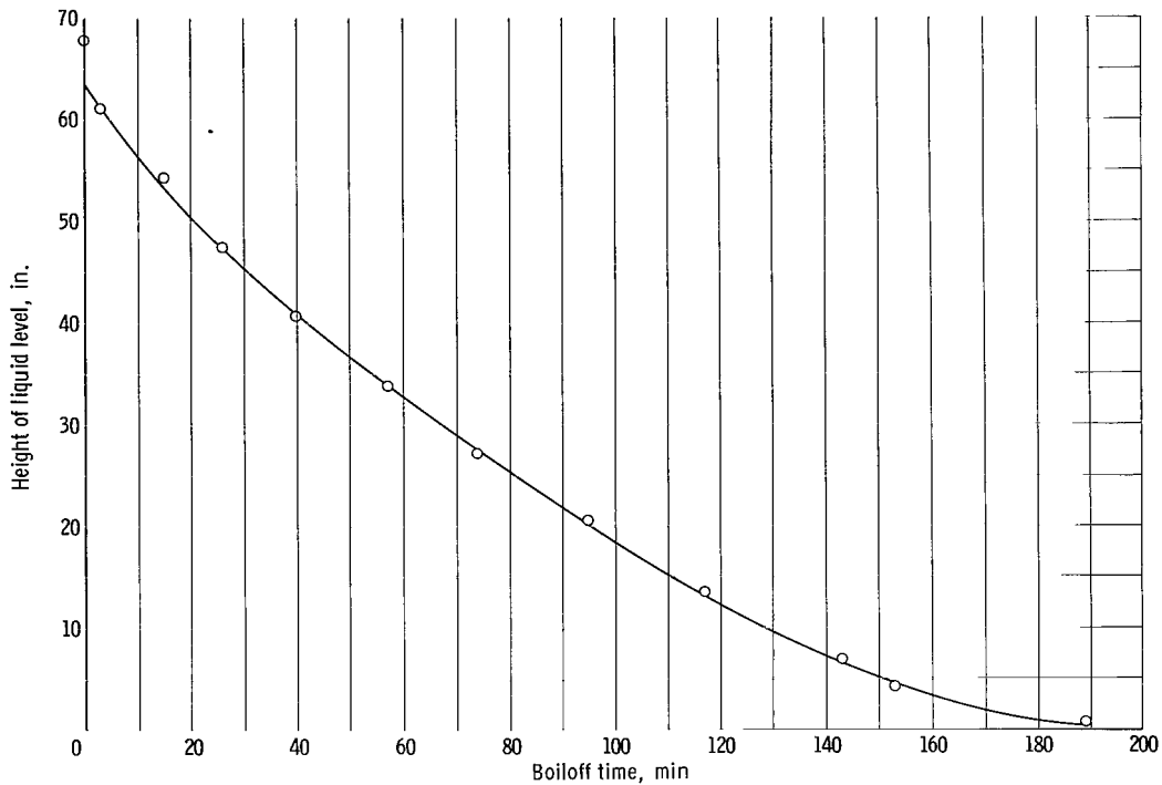
Figure 9. - Typical change in liquid level during boiloff of liquid hydrogen from sealed-foam-insulated tank.
