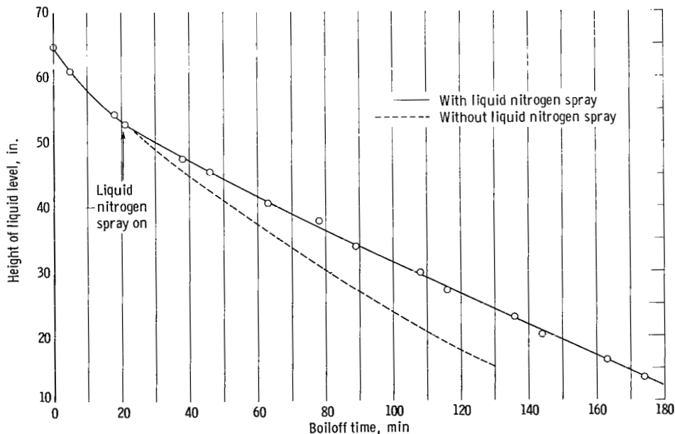
Figure 17. - Change in liquid level during boiloff of liquid hydrogen from sealed-foam-insulated tank with and without liquid-nitrogen spray over insulation.
