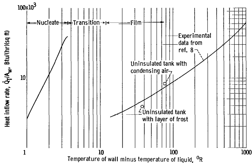
Figure 18. - Comparison of results from uninsulated tank tests with experimental data for boiling heat transfer for liquid hydrogen.
