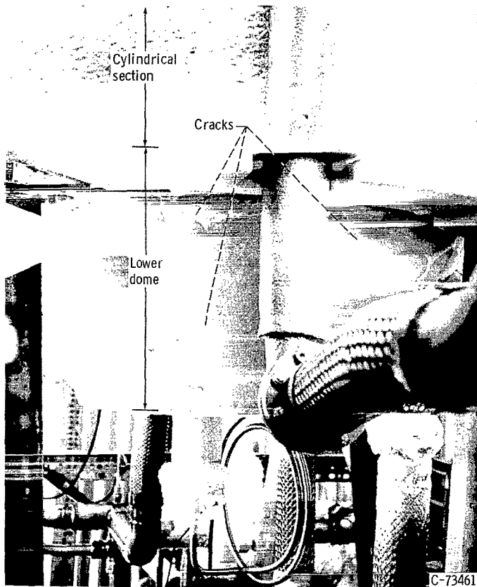
Figure 12. - Cracks in corkboard insulation (area sealed with lacquer on lower dome) following cooldown of tank with liquid hydrogen.
