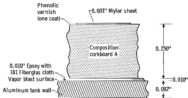
Figure 3. - Externally bonded corkboard insulation design for liquid-hydrogen fueled rocket tanks using seal against air penetration on outside surface. Insulation system weight, 0.53 pound per square foot.
