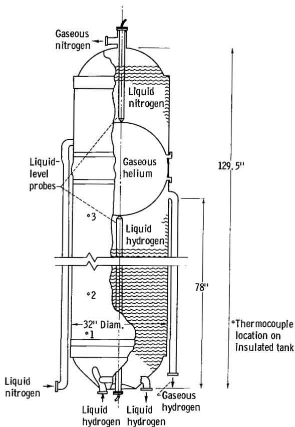
Figure 1. - Flight-weight propellant tank 1 used for corkboard insulated and uninsulated tank studies.
