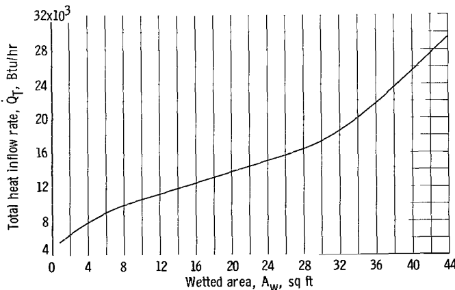
Figure 13. - Plot of total heat inflow rate against wetted area for boil-off tests of corkboard-insulated tank.
